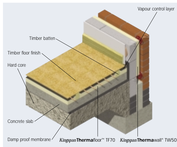
Figure 10 Underfloor Heating – Timber Floor on Batters
