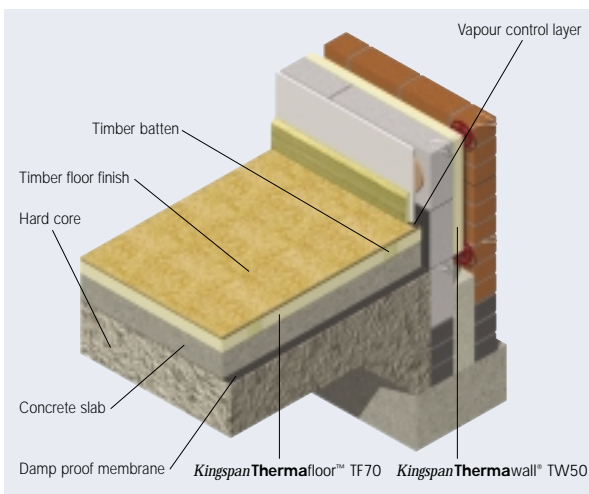
Figure 9 Timber Floor on Batters
